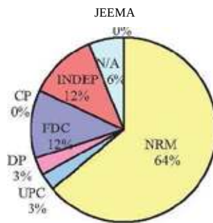
Figure 2: Party Membership
